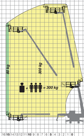
ROTO 40-26 MCSS AERIAL WORK PLATFORM THROUGH 360°
