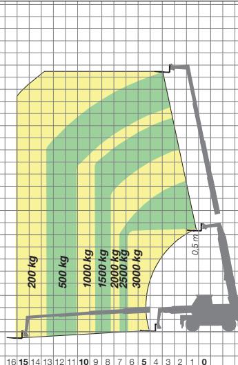
ROTO 40-26 MCSS FORKS ON TYRES - FRONT
