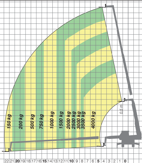
ROTO 40-26 MCSS FORKS ON STABILIZERS THROUGH 360°
